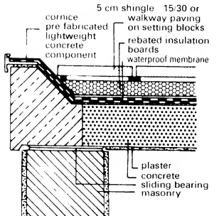
3 Flat roof construction
